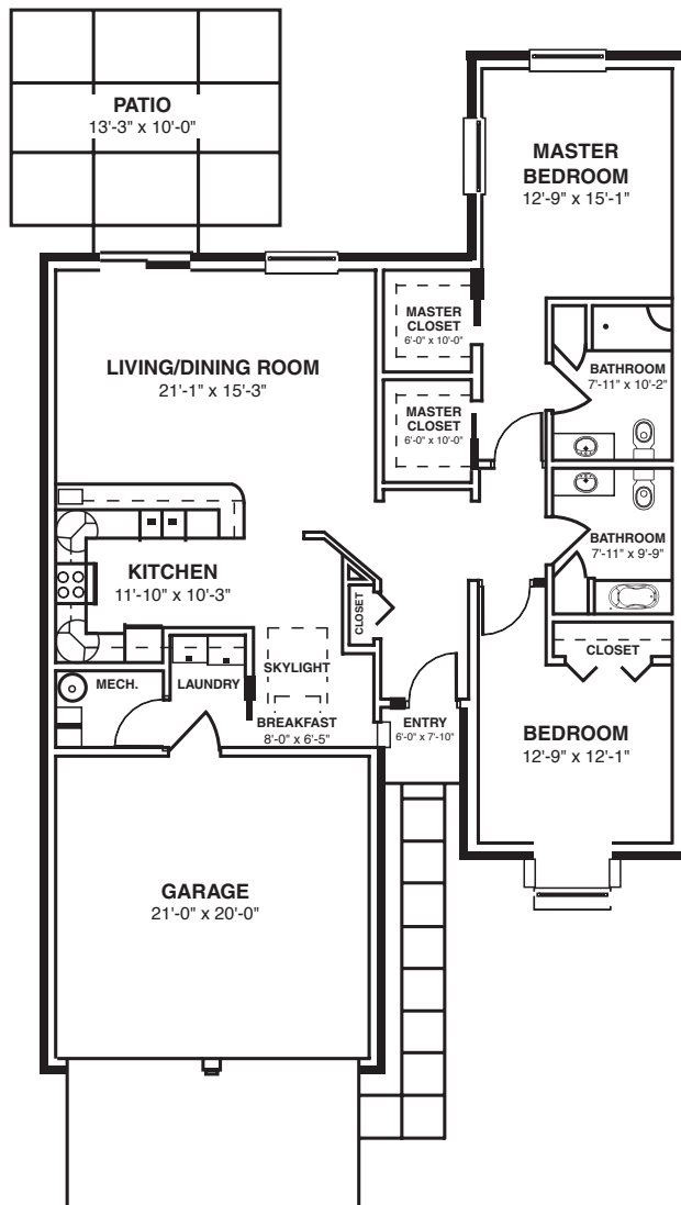
FLOOR PLAN
